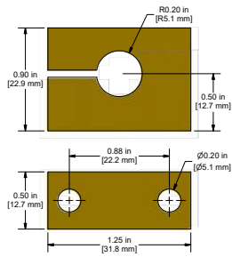
Phenolic proximity probe mount, clamping version, with clearance hole for M10 threaded probe case
