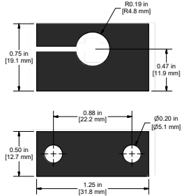
Aluminum proximity probe mount, clamping version, with clearance hole for \frac{3}{8} -24 threaded probe case
