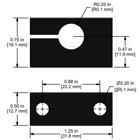
Aluminum proximity probe mount, clamping version, with clearance hole for M10 threaded probe case
