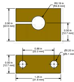
Phenolic proximity probe mount, clamping version, with clearance hole for \frac{3}{8} -24 threaded probe case
